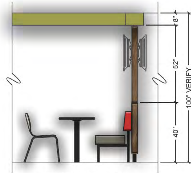
J ELEVATION 1/4" = 1'-0"
