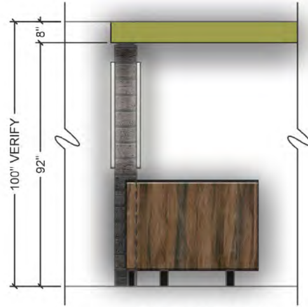
G ELEVATION 1/4" = 1'-0"
